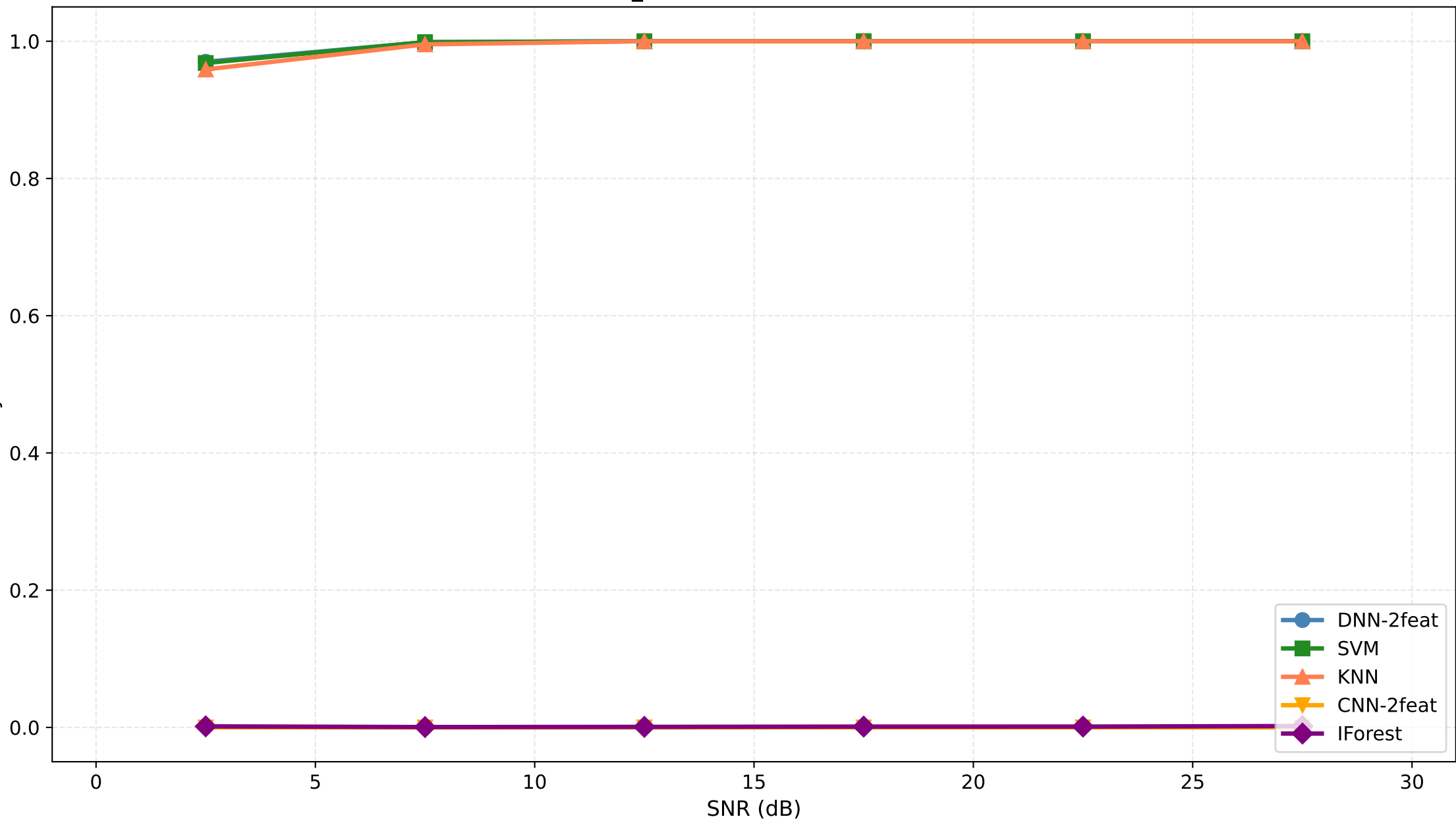
P_D vs SNR ( \alpha = 10^{-7} )
